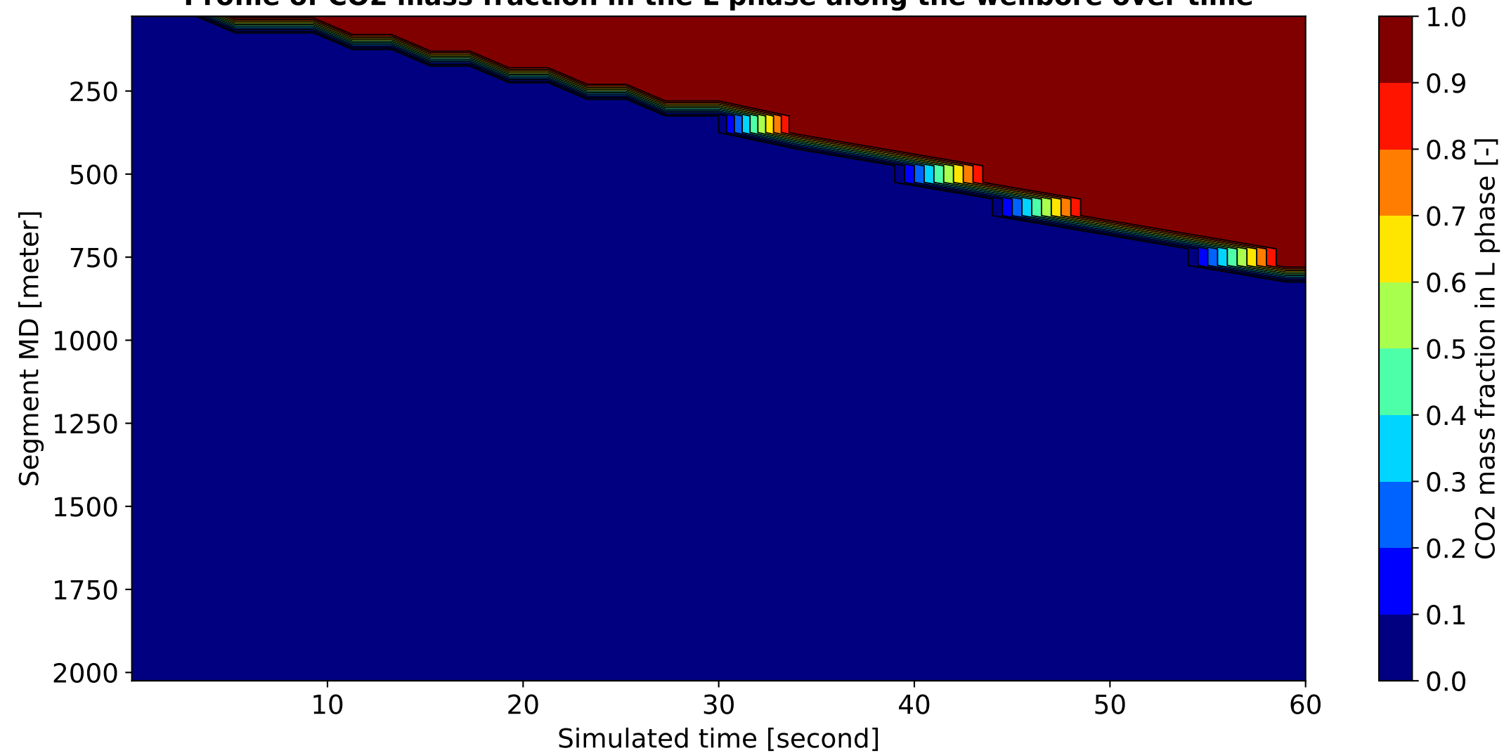
Profile of CO2 mass fraction in the L phase along the wellbore over time
